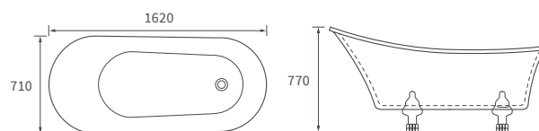
TIVERTON FLOORSTANDING BATH
