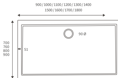
LOW PROFILE RECTANGULAR TRAYS
