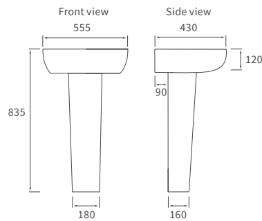
BASIN WITH FULL PEDESTAL 555 x 430mm
