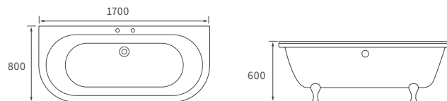
FINCHLEY BATH
