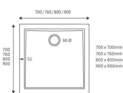
LOW PROFILE SQUARE TRAYS
