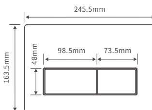
SQUARE FLUSHPLATE
