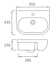
SEMI RECESSED BASIN 555 x 435mm
