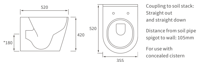
RIMLESS BACK TO WALL PAN
