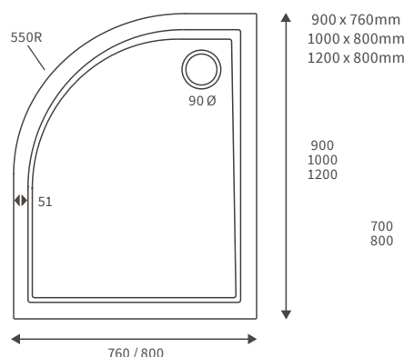
LOW PROFILE OFFSET QUADRANT TRAYS
