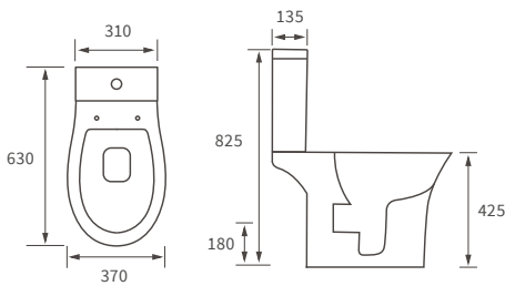
CLOSE COUPLED PAN AND CISTERN
