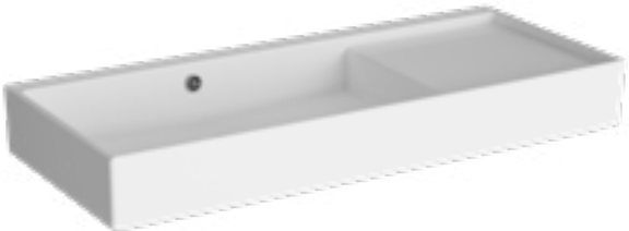
Compact basin, oTH, 90cm • White £573 – 7405B003-0012 H: 120mm W: 900mm P: 380mm
