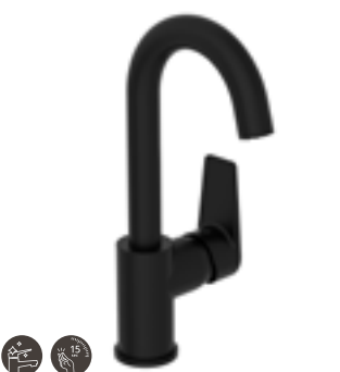
Flow Square basin mixer with swivel spout H: 280mm P: 114mm
