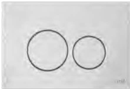
Origin mechanical flush plate compatible with all frames H: 165mm W: 244mm P: 8mm
